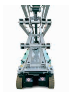
New design of the chassis which allows easy cleaning and ensures protection to the components
